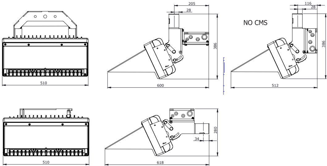
FL820-1-F (SINGLE MODULE FULL CUT OFF)
