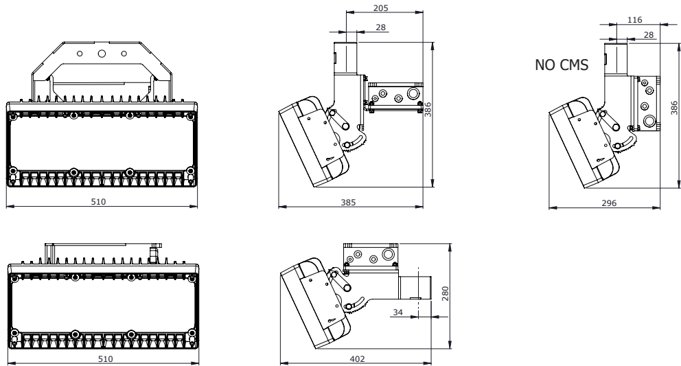
FL820-1-P (SINGLE MODULE PROJECTOR)
