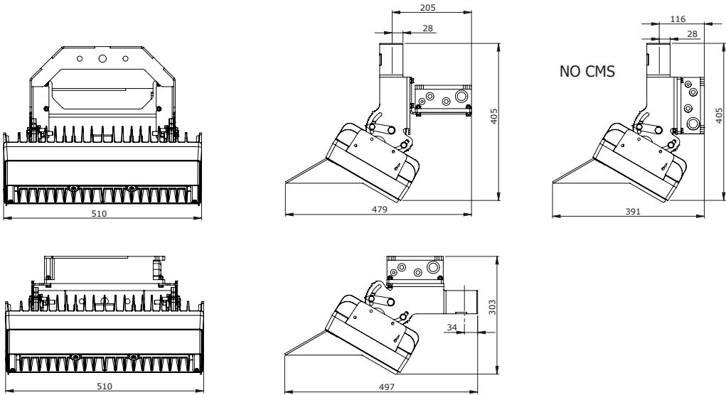
FL820-1-L24 (SINGLE MODULE - L24 30° COWL)
